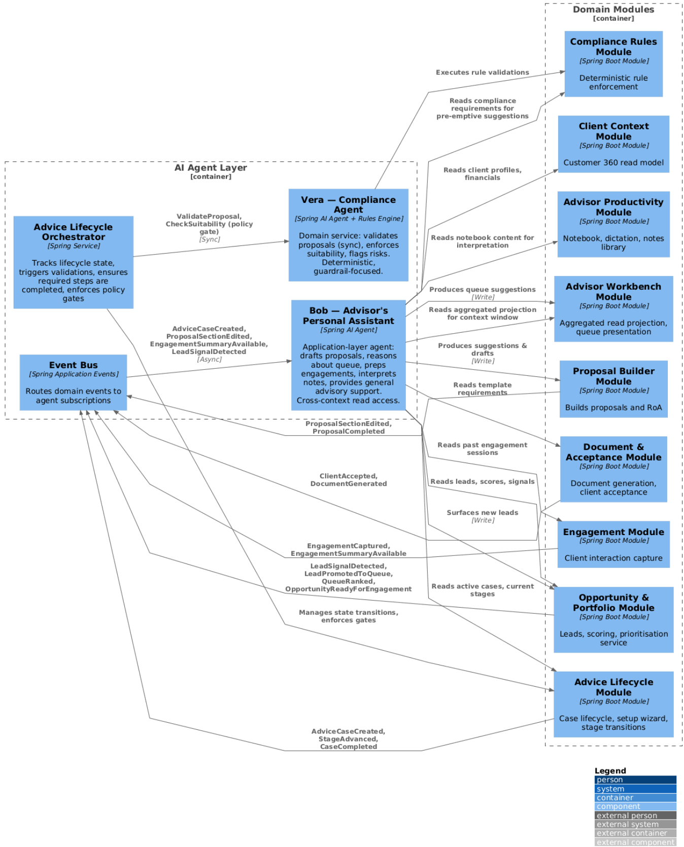
AI Agents & Orchestration — Component Diagram
